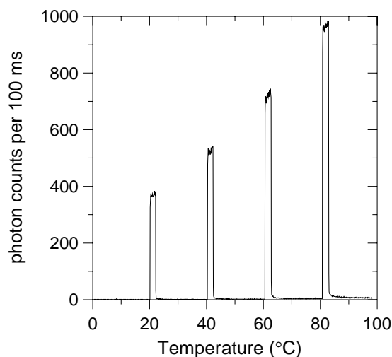
Figure 1: Photon emission vs. temperature for K8
