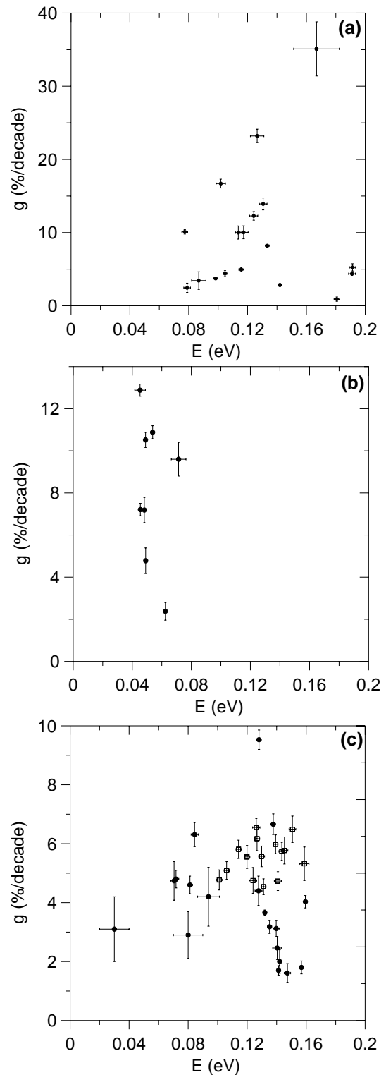
Figure 4: Fading parameter vs. activation energy for a) alkali feldspars, b) plagioclase feldspars and c) K-feldspar grains from sediment - open squares for Canadian prairie sediments, closed circles for other sediments
