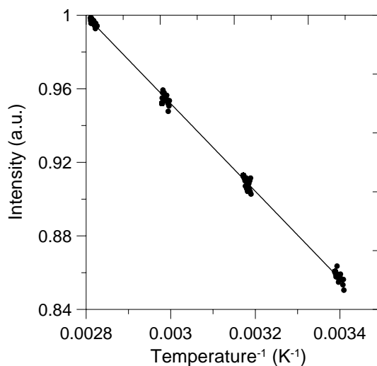
Figure 2: Fitted data used to extract E for K8
